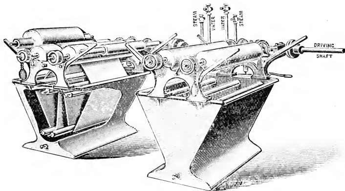
FIG. 18.—Dye-jiggers.
